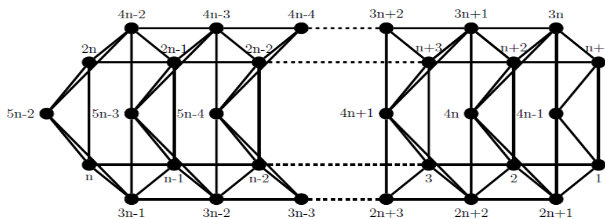
Figure 1: T(L_n)
