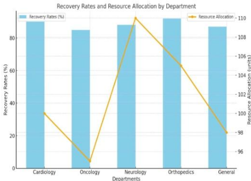
Figure 1: Visualisation analysis
