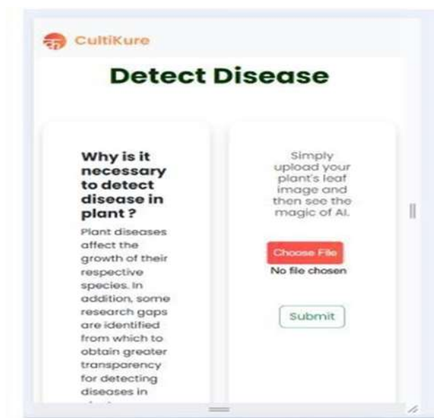
Fig.9. Uploading image
