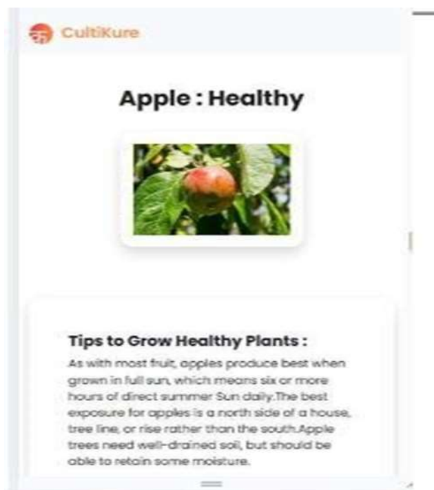
Fig.10. predicted result
