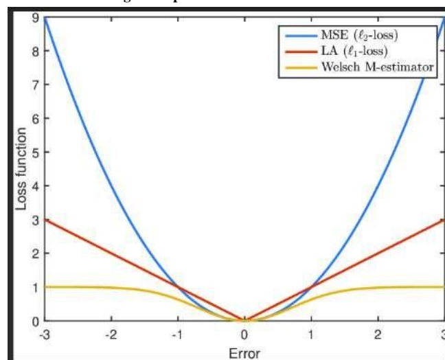
Fig : Comparson of Different Loss functions.
