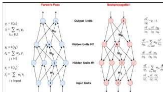
Fig : Forward Pass and Backpropagation in a neural Network.
