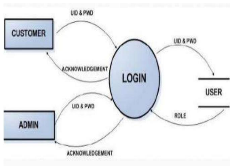
Figure 3: Data Flow chart
