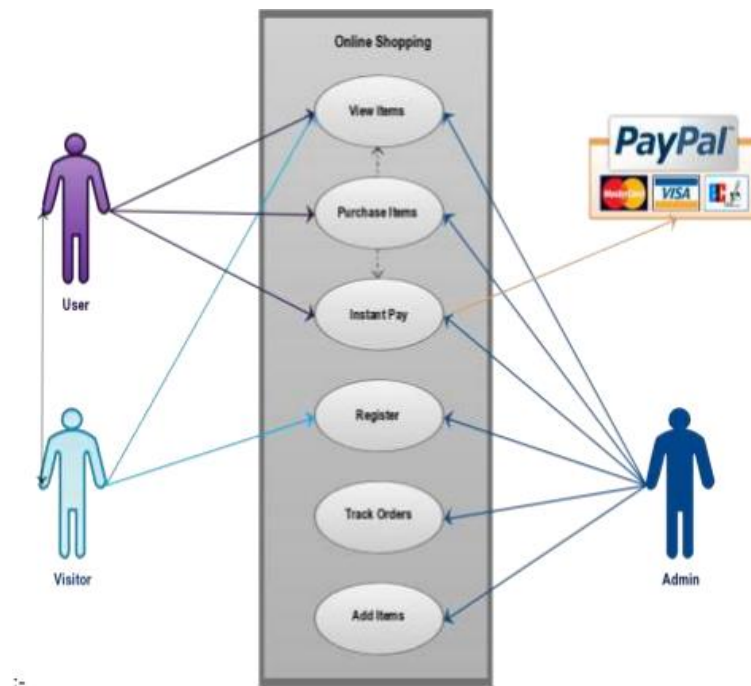
Figure 2: Relation Chart. Data Design
