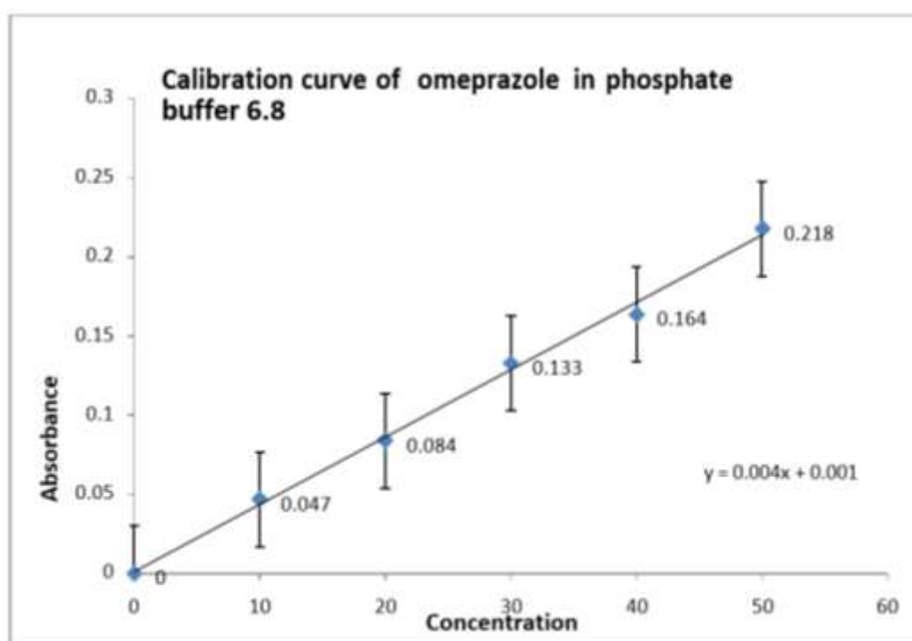
Figure 3: Calibration graph of Omeprazole in phosphate buffer pH 6.8 at 300nm Omeprazole in phosphate buffer pH 6.8 follows the Beer–Lambert’s law in the concentration range of 10-50 µg/ml.
