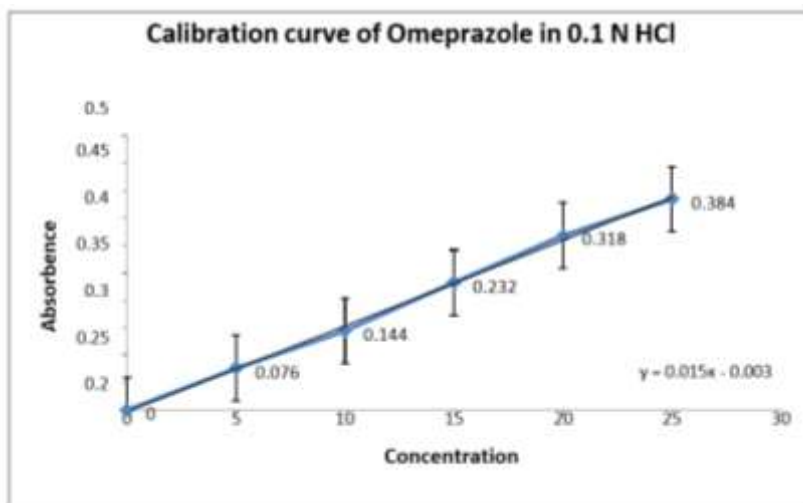
Figure 4: Calibration graph of Omeprazole in pH 1.2 HCl buffer at 300nm
