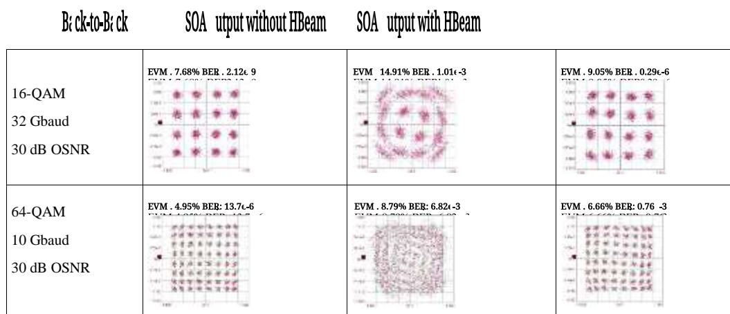
Fig. 2. Illustration of the use of SOA in coherent communication : Constellations for output of SOA for 16-QAM (top) and 64-QAM (bottom) formats in three situations (back-to-back in left column, with SOA but no holding beam in middle column and with SOA with holding beam in right column) when the drive current was 350 mA.
