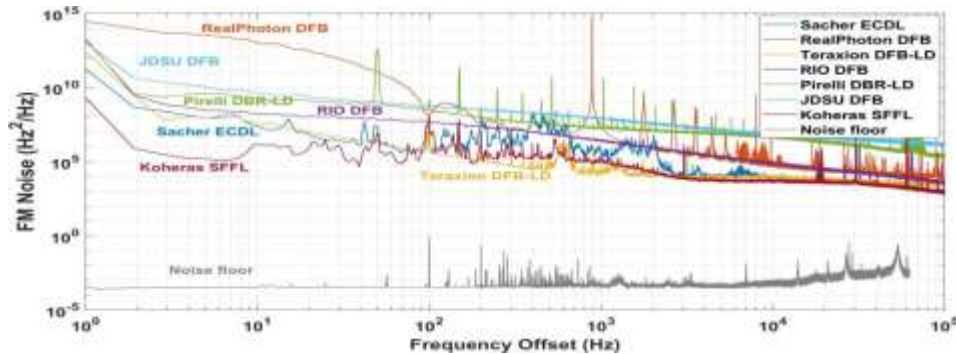
Fig. 6. FM noise spectrum of different types of narrow linewidth laser diodes. laser under test shown in Figure 7), the estimated linewidth is 10 kHz is matching closely with the datasheet. This phase noise analyser is packaged into a prototype and hence can be easily transported for measurements. We have been carrying out prototyping at the laboratory level for other experiments as well.
