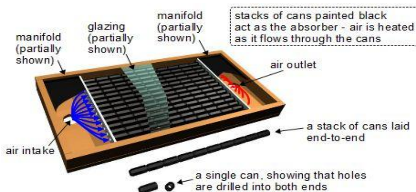
Fig. 1 Solar Air Heater
