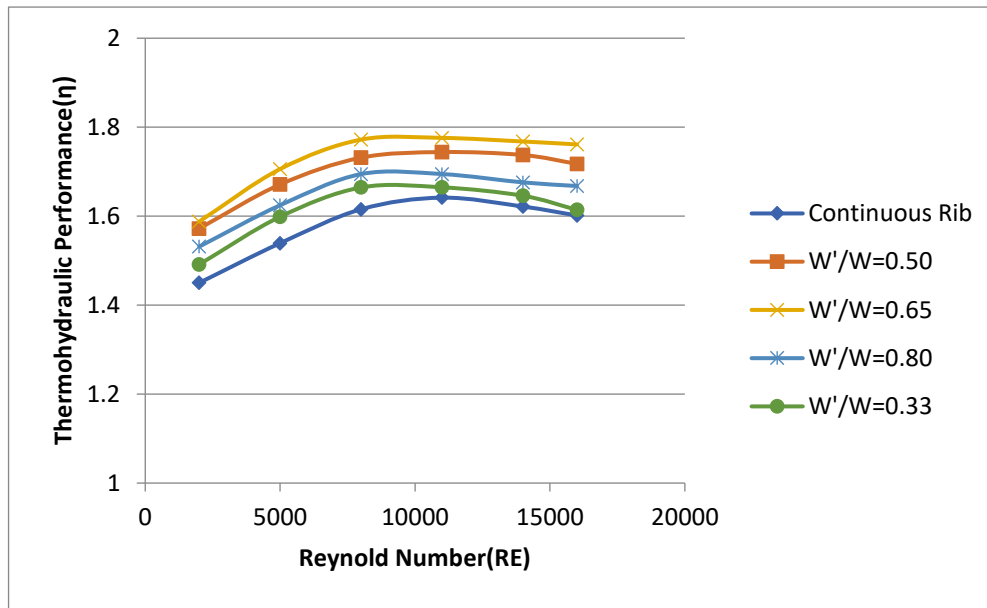
Fig.5 Thermo-hydraulic performance parameter as a function of Reynolds
