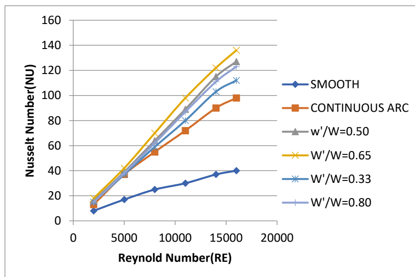
Fig. 4. Variation of Nusselt number with Reynolds number for different Values of relative gap position ( W'/W ).
