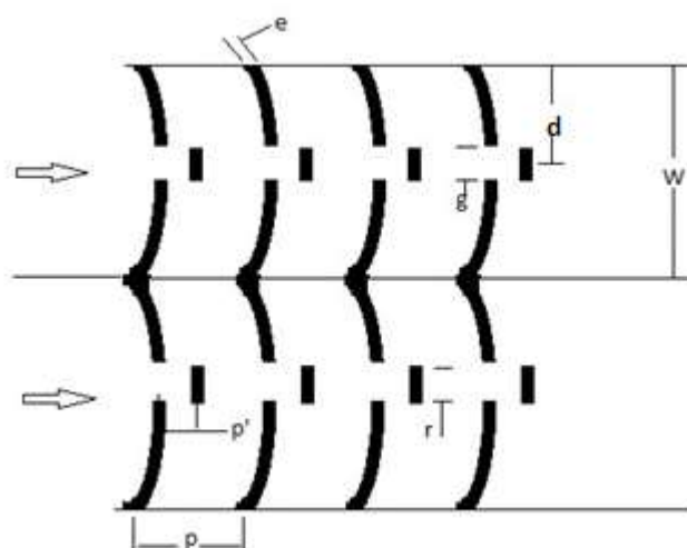
Fig. 2 Schematic diagram of Broken arc rib with stagger Piece
