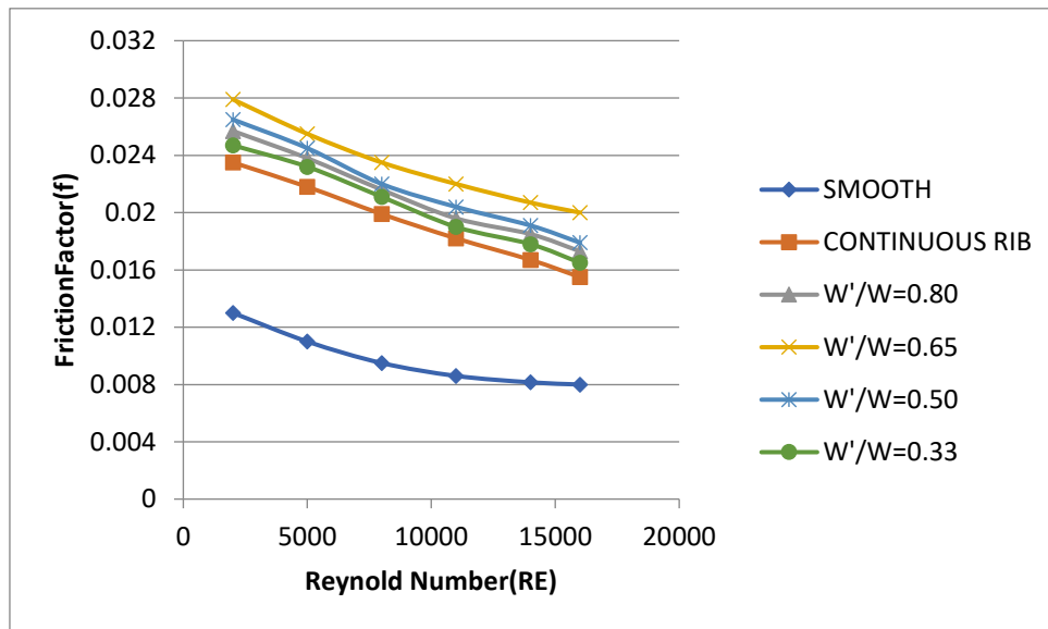
Fig. 5 Comparison between Friction factor and Reynolds number at different gap position ( W'/W )
