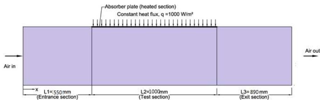
Fig. 1. Showing the geometric dimension of the working model
