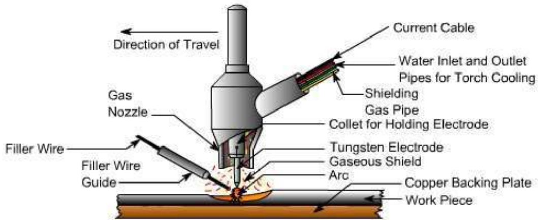
Fig. 2: Principle of TIG Welding. [Ref: 1]
