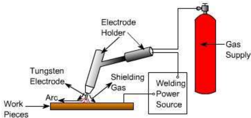
Fig 1: Schematic Diagram of TIG Welding System. [Ref: 1]
