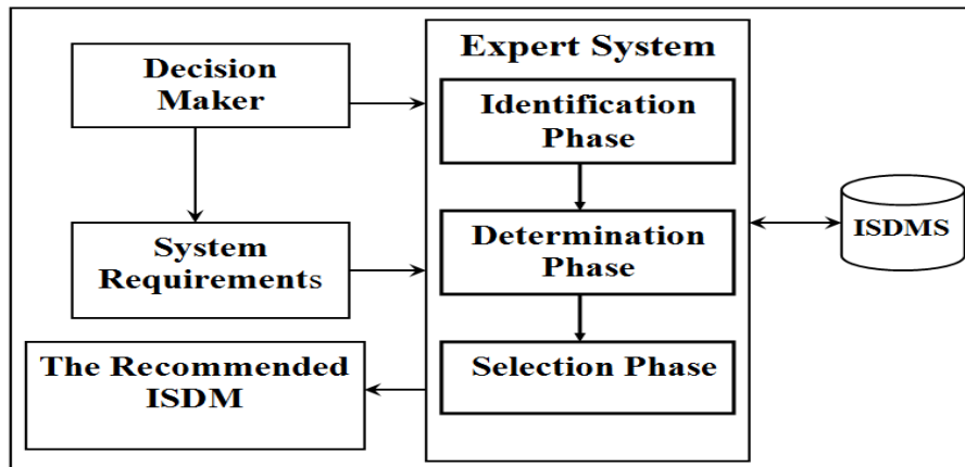
Fig 1.0: Expert System Framework
