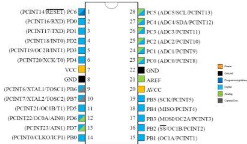
Fig.2. Pin Diagram of Atmega 328p
