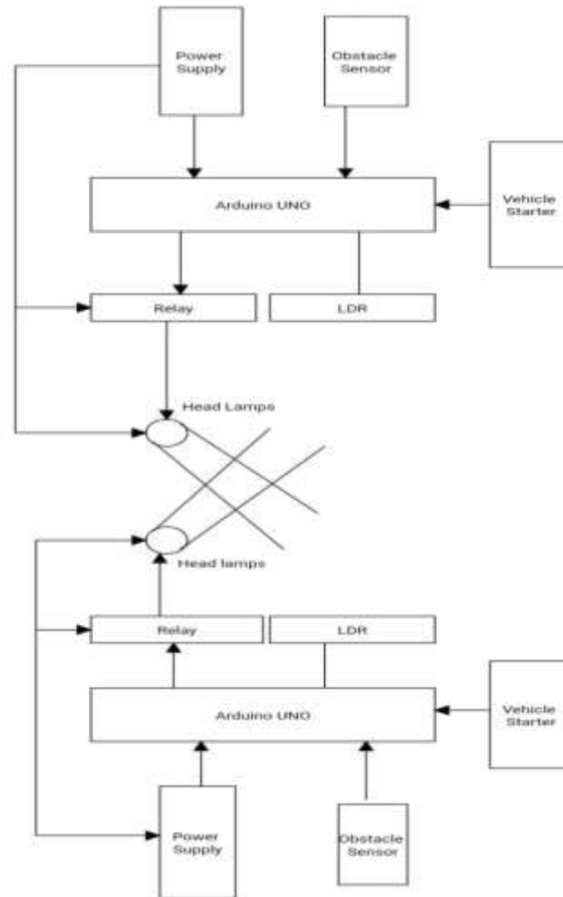
Fig.3. Working Block Diagram
