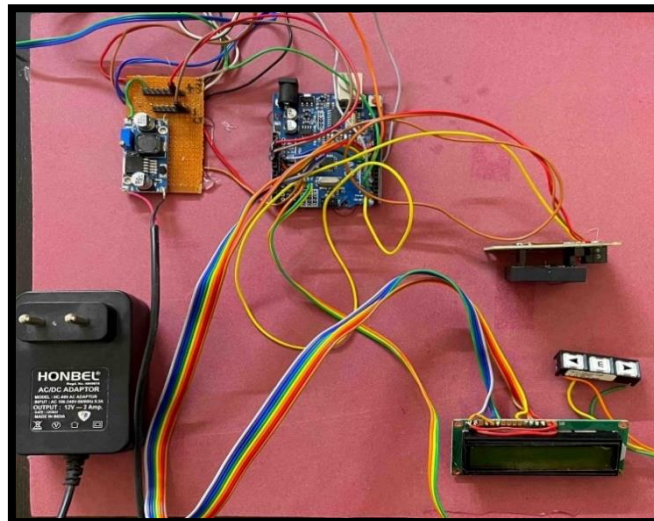
Fig.4: Experimental Setup
