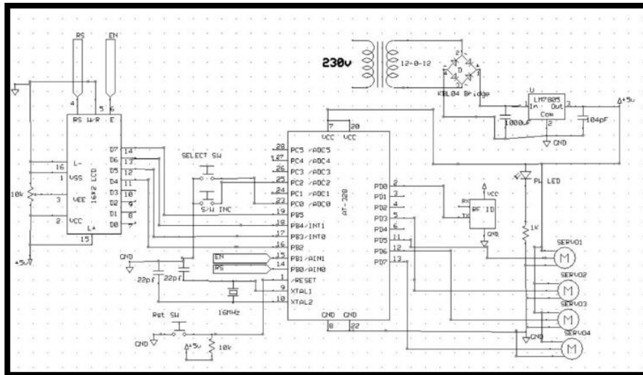
Fig.3: Circuit Diagram
