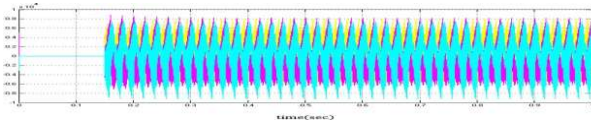
Fig. 7.12 compensating current from D-STATCOM
