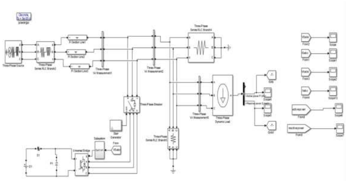
Fig. 7.1 simulink diagram without insertion of D-STATCOM
