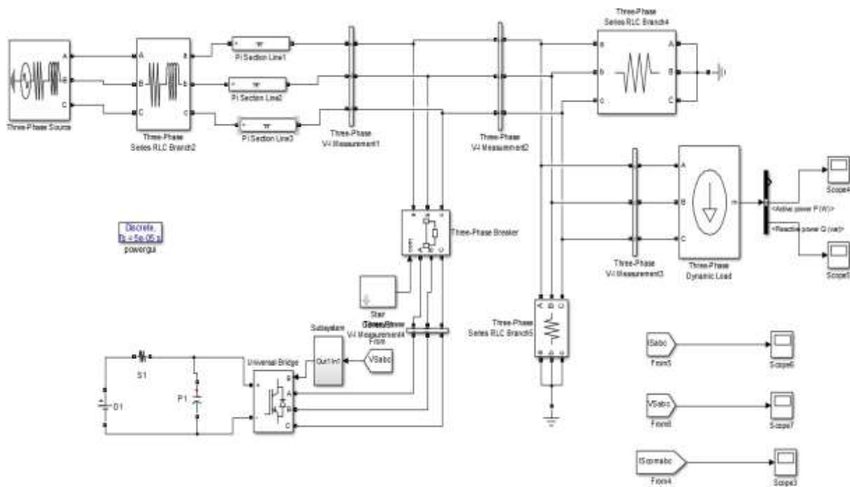
Fig. 7.9 simulink diagram with insertion of D-STATCOM
