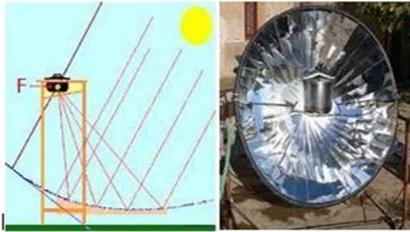
Figure 1. Solar panel cooker
