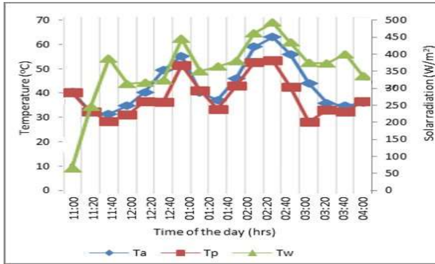
Figure 6. Solar cooker performance curve during heat test of water
