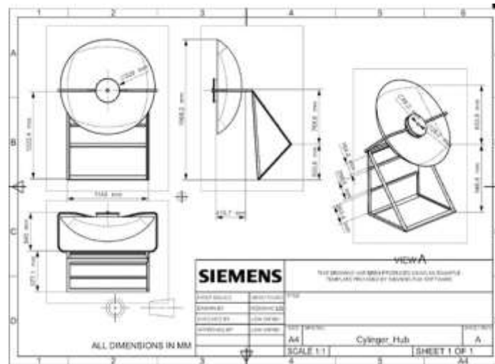
Figure 3. Geometrical drafting of cylindrical model solar cooker
