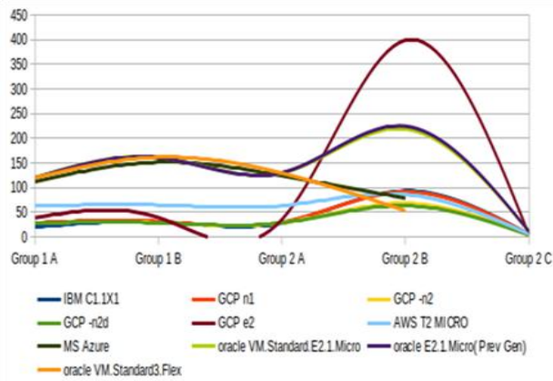
Figure 1: Comparison of the VMs on the basis of Time Taken
