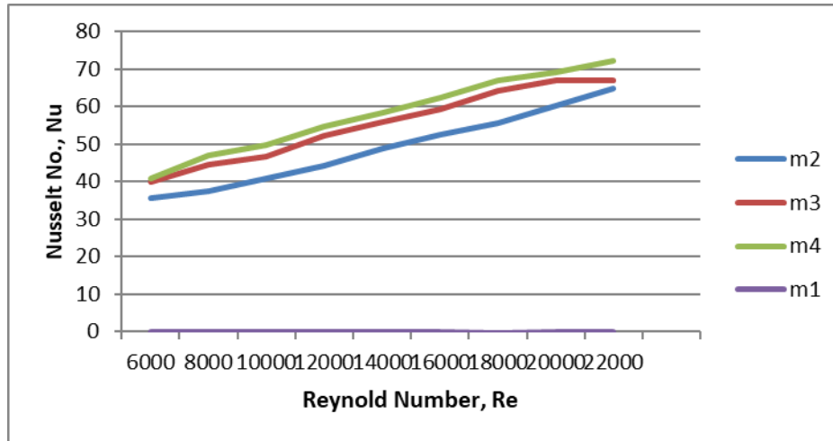
Fig 3 Plot of Nusselt number vs Reynolds Number
