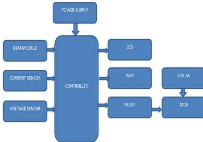
Fig no.1: electric vehicle battery charging station using iot diagram
