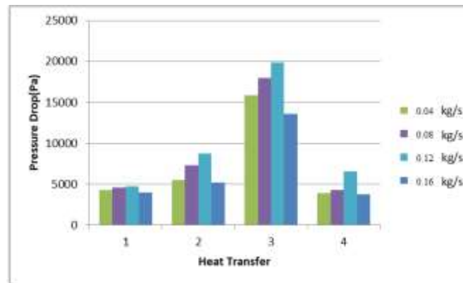
Fig. 4 Graph of Correlation of Pressure Drop
