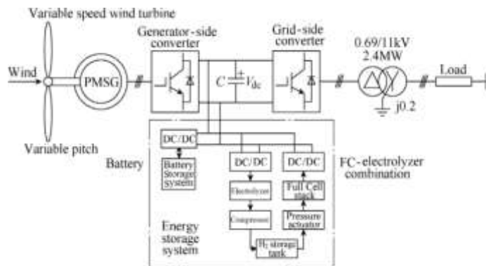
Fig.1 Block diagram of a VSWT based on direct-drive PMSG, full-scale power converter and ESS
