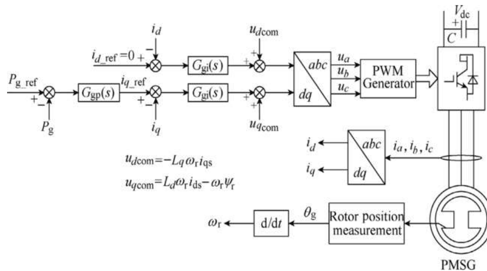
Fig.9. Block diagram of the control structure for generato-side converter
