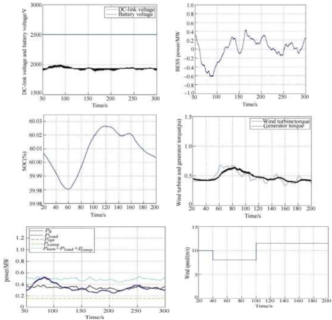
Fig.13 The performance of the system for step change of wind speed
