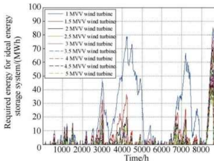
Fig.3 Energy required for ideal energy storage system
