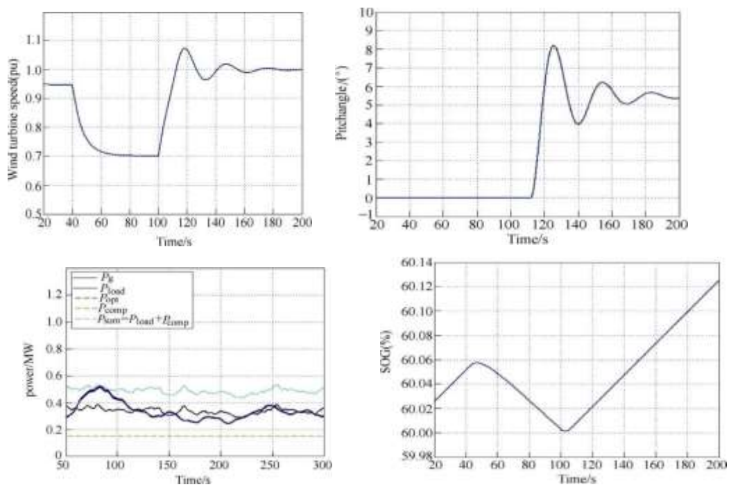
Fig.12 The performance of the stand-alone wind turbine system
