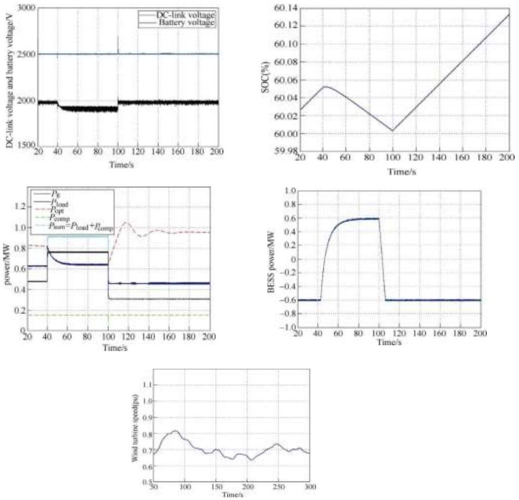
Fig.12 The performance of the stand-alone wind turbine system
