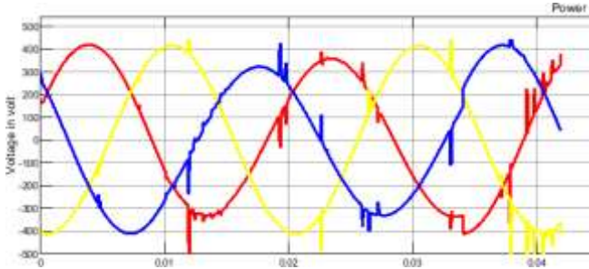
Fig 8. Three Phase voltage at the output of three phase inverter when irradiance =1000W/m 2
