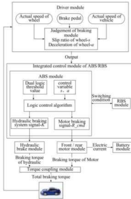
Fig 4: Braking coordination process
