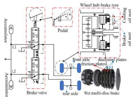
Fig3: Break circuit
