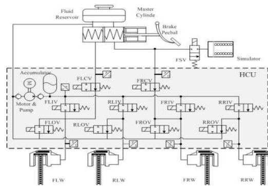
Fig 5: The structure of the EHB
