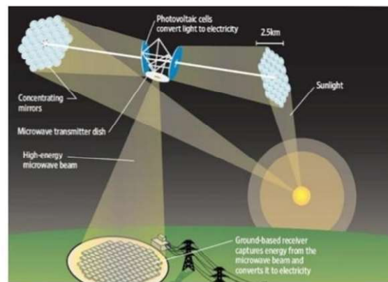
Fig 1: Microwave concept satellite
