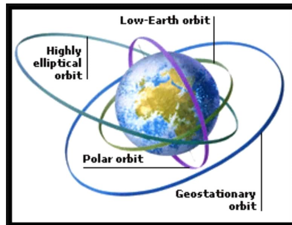
Fig 3: Different Orbits
