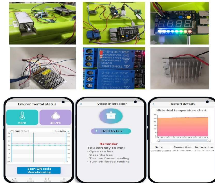
Fig. 3. Real object diagram of system
