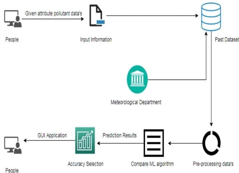
Figure 1.1: System Architecture Of The Proposed System
