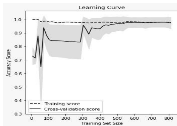
Figure 5.2: Naïve Bayes Accuracy graph
