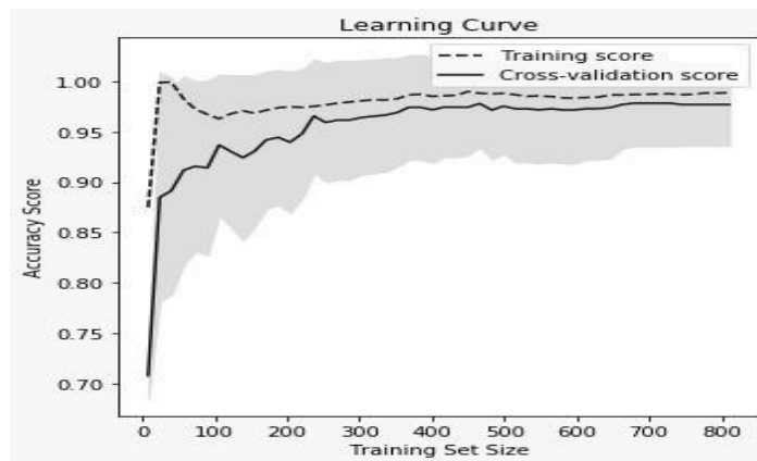
Figure 5.6: KNN Accuracy graph
