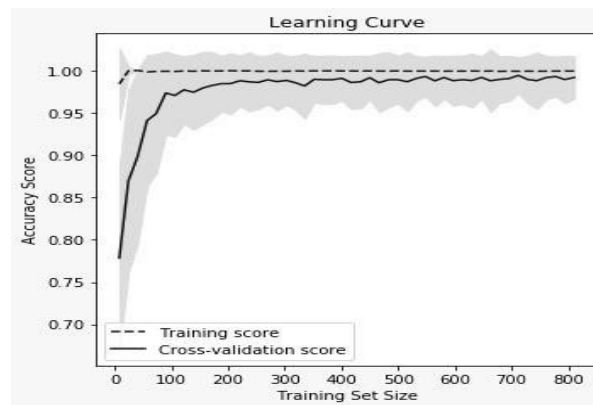
Figure 5.4: Random Forest Accuracy graph
