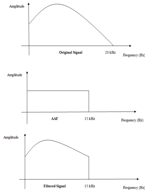
Fig.1 Illustration of the information loss due to AAF.
