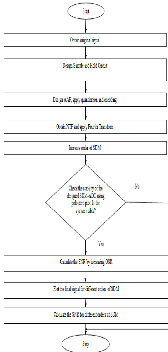
Fig.4: Flow Chart for Proposed System
