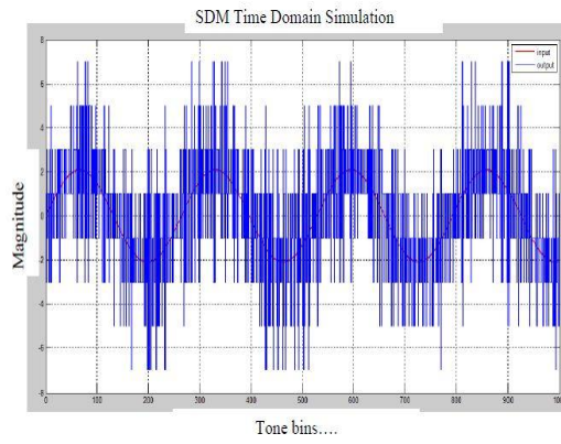
Fig.9 Third order t-d response
