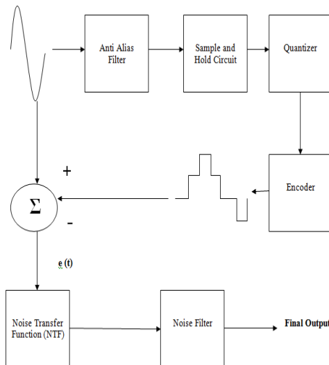
Fig.3 Block Level Implementation of Proposed System.
