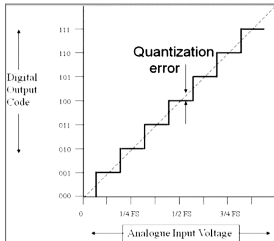
Fig.2 Variation of Quantisation error as a function of signal voltage
