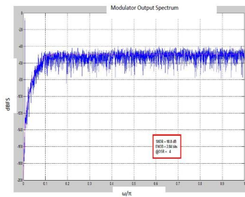
Fig.12 Fourth order f-d response
