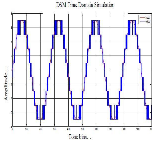
Fig.5 First order t-d response
