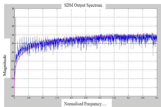
Fig.8 Second order f-d response
