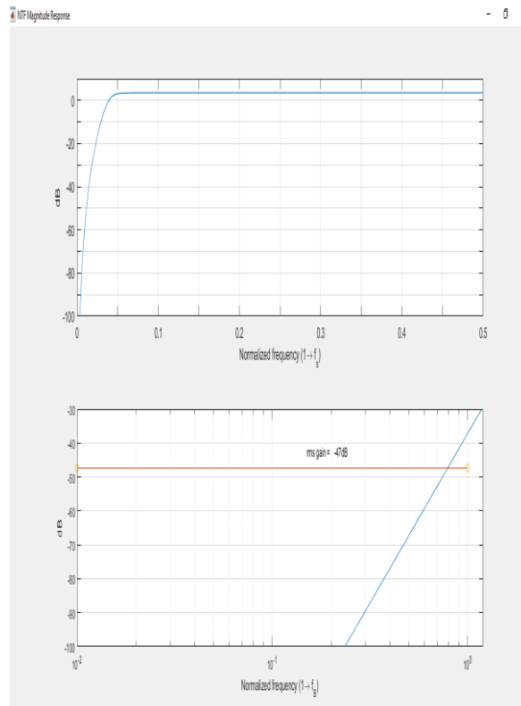
Fig.14 Gain plot for 5 th order
