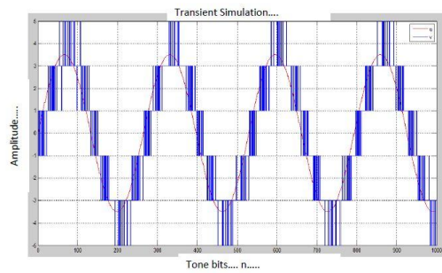
Fig.11 Fourth order t-d response
