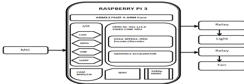
Fig1:Blockdiagramof home automation using raspberry-pi
