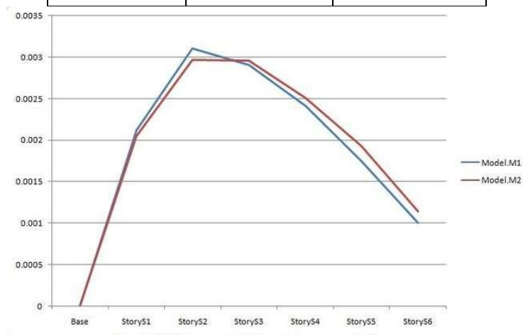
Fig 26 Storey drift (for 6 storey model)
