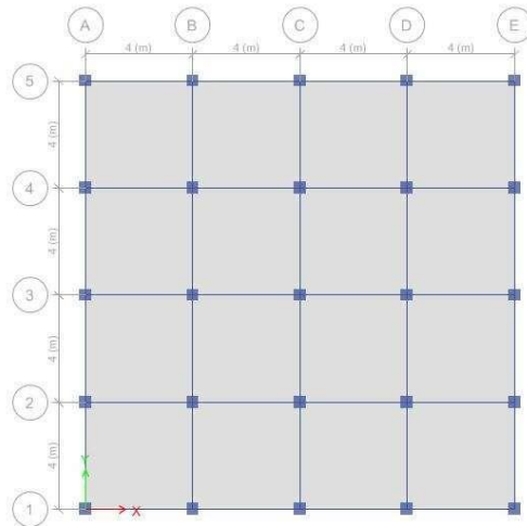
Fig. 5 Plan of Model 2 (1-2 Storeys)
