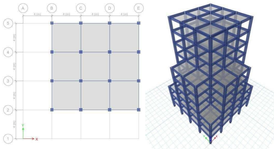
Fig 19 Modelling
