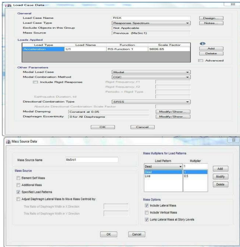
Fig 23 Dynamic analysis procedure
