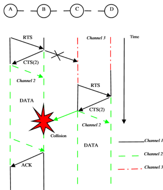
Fig.2 Multichannel collision Problem in MAC
