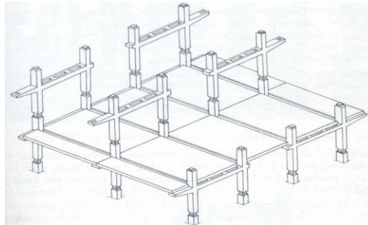
Fig -10: A Skeleton construction
