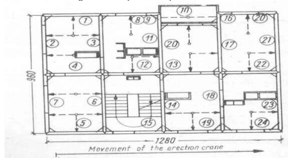
Fig 13 Erection schedule of a PBU type large-panel building, numbers in circles denote the sequence of assembly, R = stays
