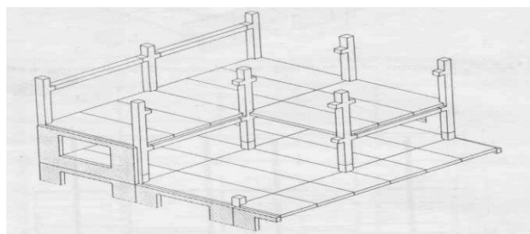
Fig -7: Diagram of a skeleton structure consisting of prefabricated columns and beams
