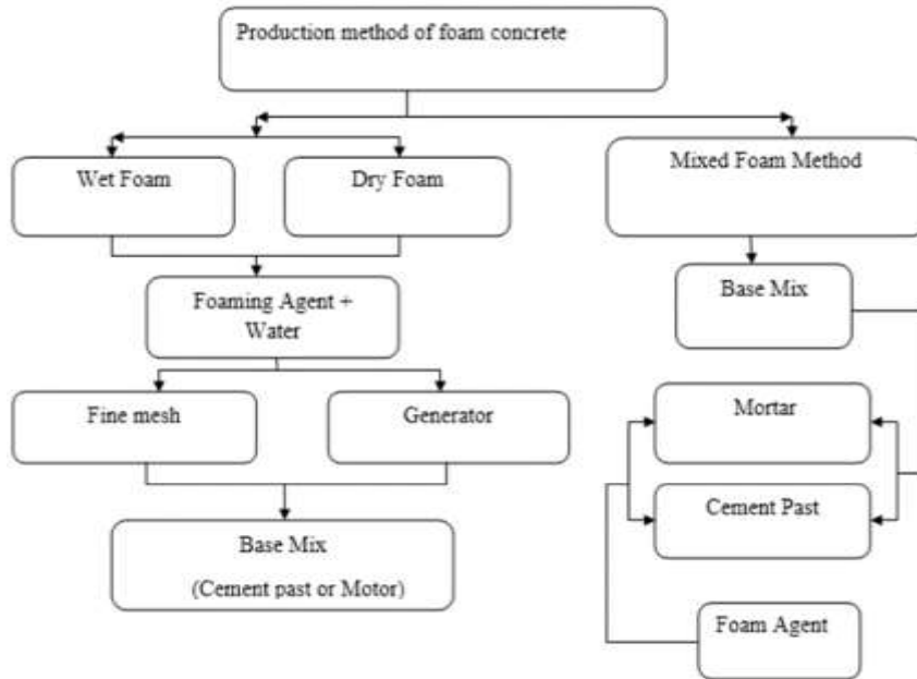
Fig. 1 - Method of preparation of foamed concrete
