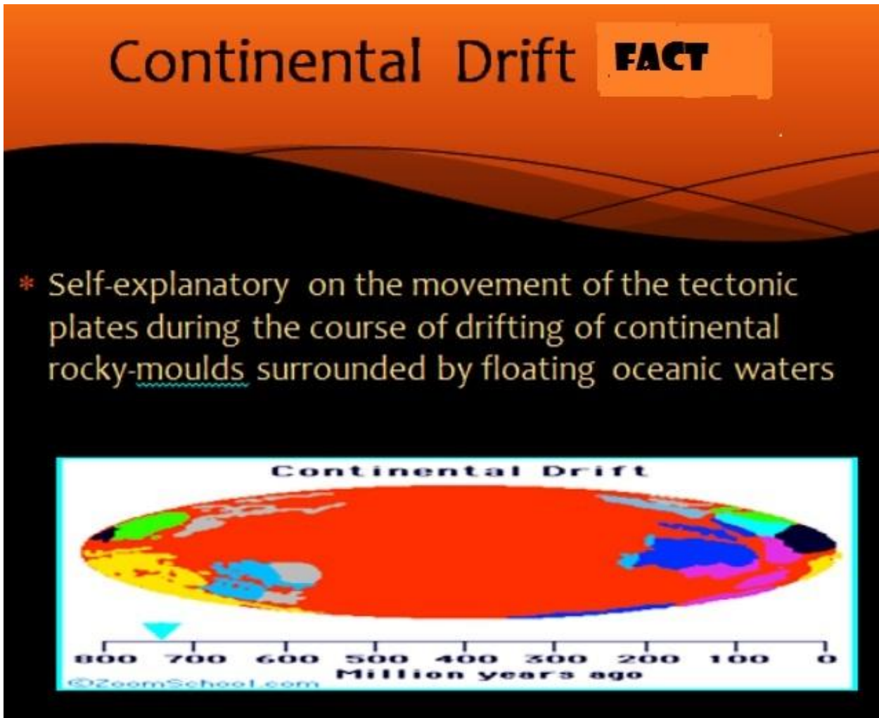
Splitting rocky-moulds through tectonic plate shift
