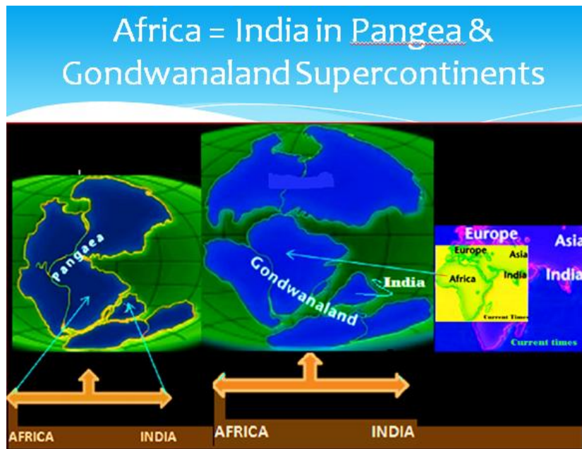
Fig 5. Pangea & Gondwana rock-slides
