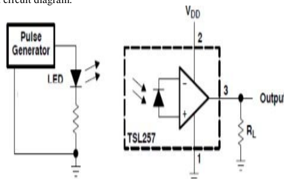
Figure 8: The Test Circuit Diagram
