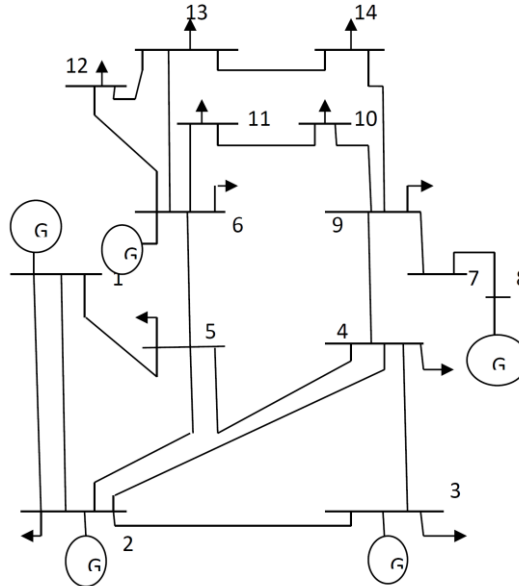
Fig 3:- IEEE 14 BUS SYSTEM
