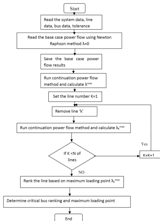
Fig 2:- Flow chart for optimal power flow
