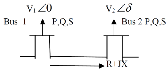
Fig. Two-bus power system model.
