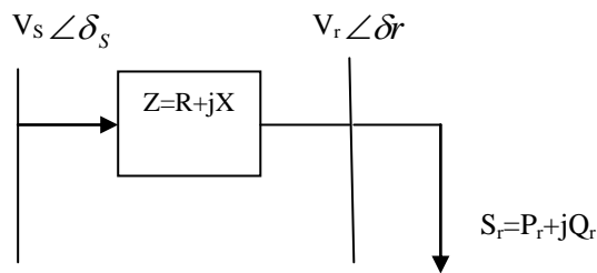
Fig1:- Two bus system
