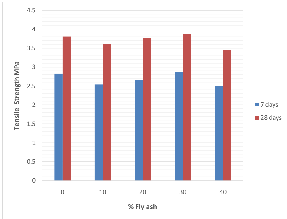
Figure 2 : Split Tensile strength of Fly ash for 7 and 28 days
