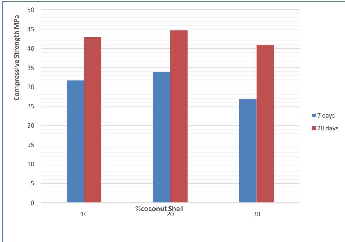
Figure 3 : Compressive strength of Fly ash and Coconut Shell for 7 and 28 days
