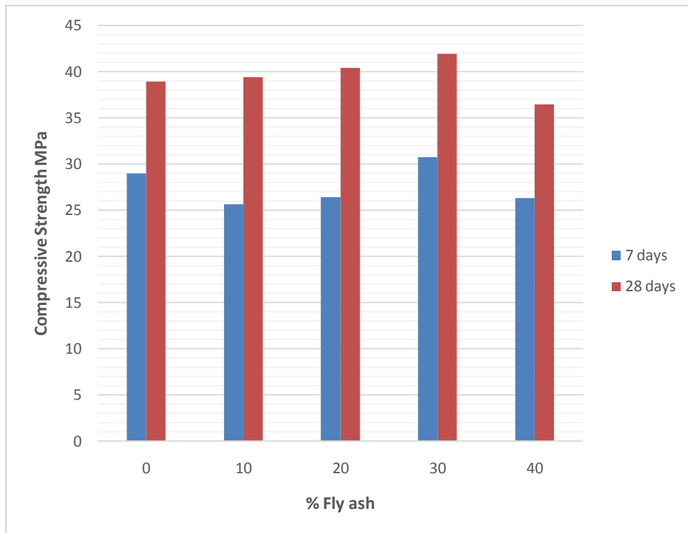
Figure 1: Compressive strength of Fly ash for 7 and 28 days
