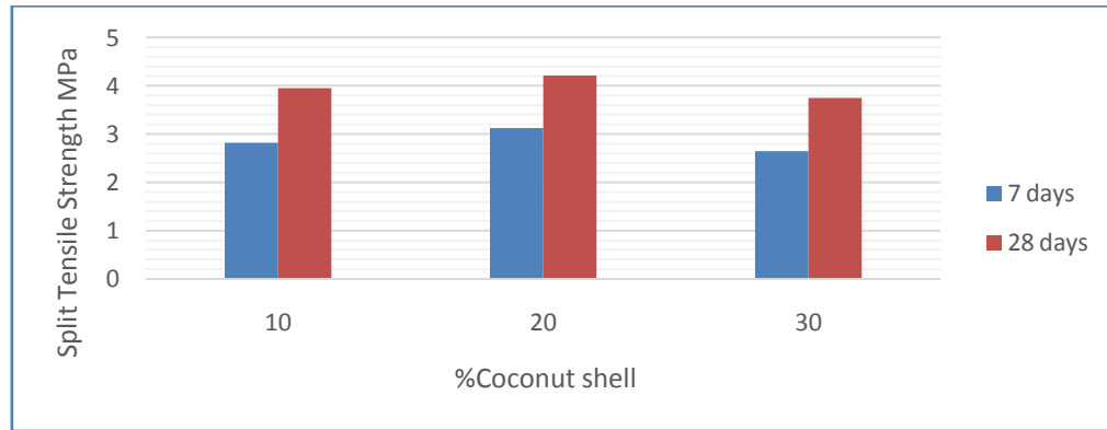
Figure 4: Split Tensile strength of Fly ash for 7 and 28 days
