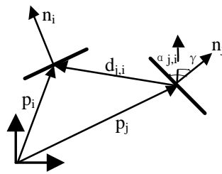
Figure 2 Local convexity
